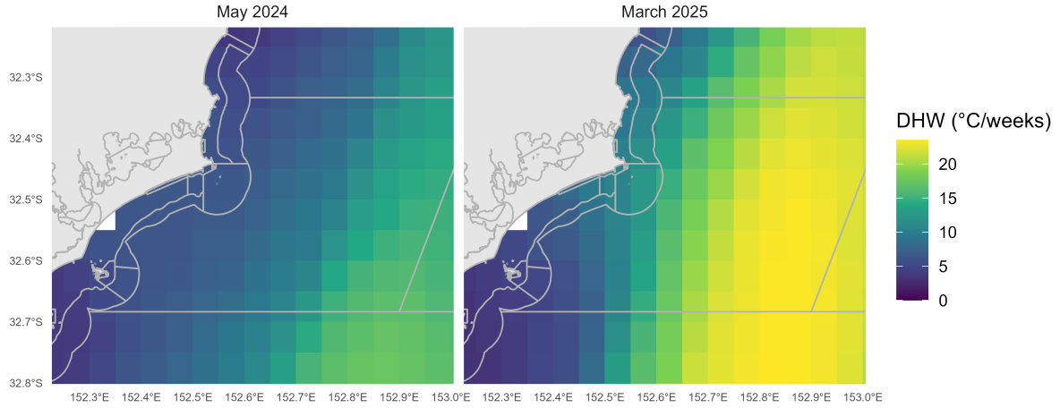
Figure B.4: Maximum Degree Heating Weeks (NOAA \geq 4 ) at the scale of the Hunter Marine Park. Heatmap values representing high (yellow) and low (blue) monthly Degree Heating Weeks (DHW) for the two most recent marine heatwave periods on record. Grey polygons represent State spatial management and Australian Marine Park boundaries.
